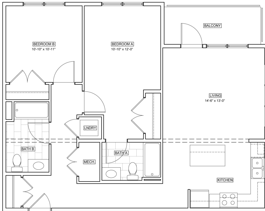
UNIT PLAN E AREA = 1,030 sf
