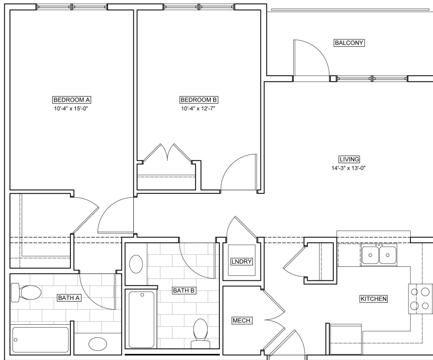
UNIT PLAN A AREA = 990 sf
