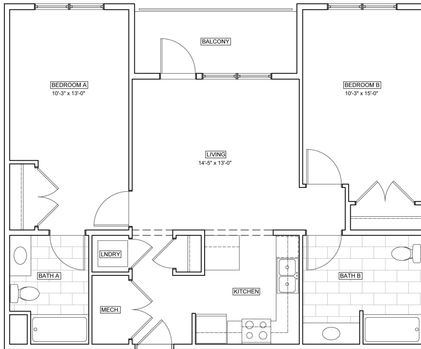
UNIT PLAN B AREA = 990 sf
