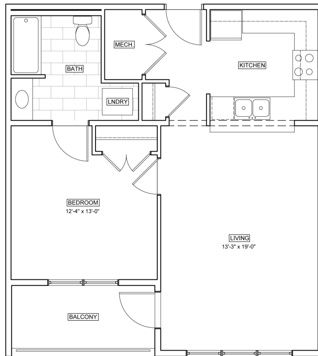
UNIT PLAN J AREA = 714 sf
